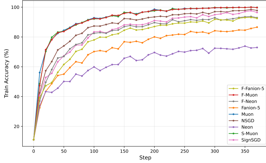
(a) Training accuracy
