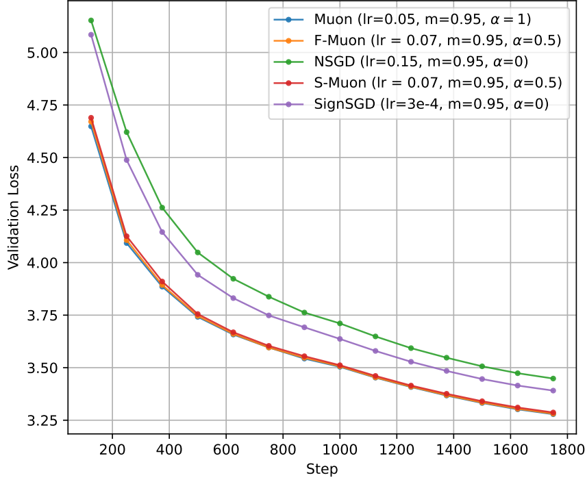
Figure 4 – The validation loss for NanoGPT.
