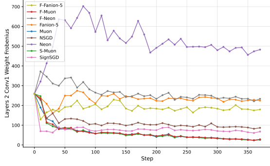
(a) Frobenius norm of layer2.conv1
