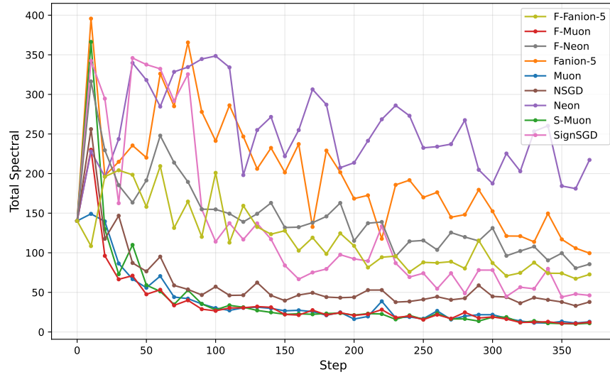
(b) Total spectral norm
