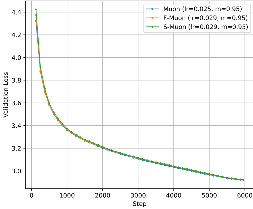
Figure 5 – The validation loss for GPT-2 Medium.
