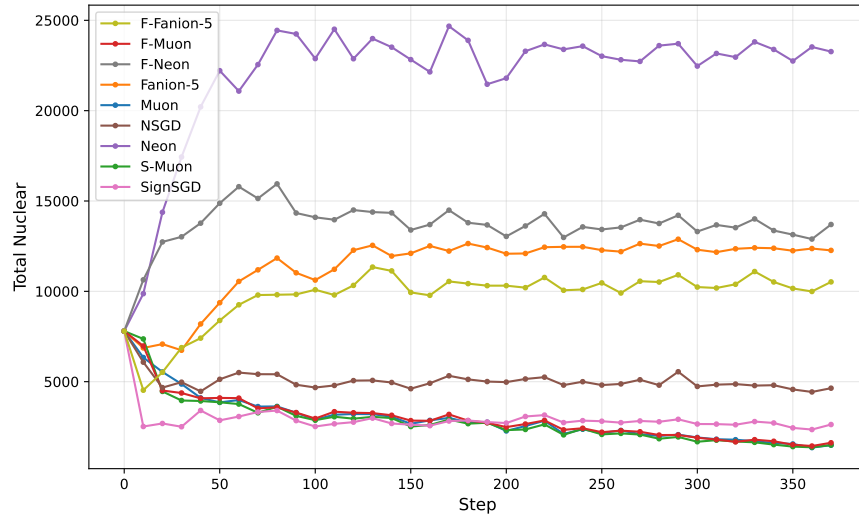
(c) Total nuclear norm
