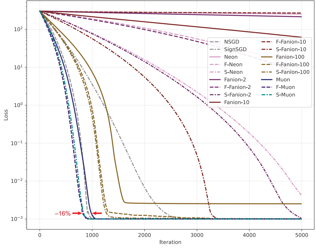
(a) The loss
