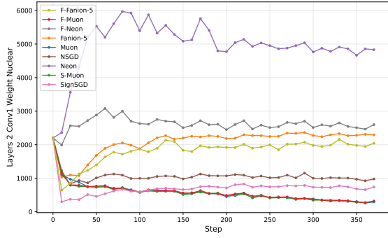
(e) Nuclear norm of layer2.conv1
