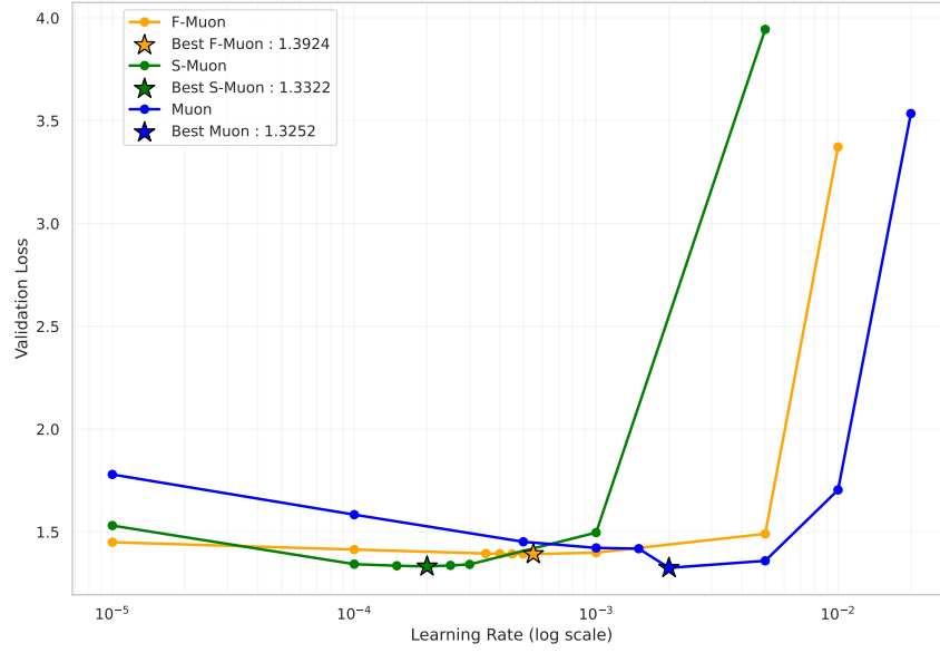
Figure 6 – Comparison of validation loss for Muon, F-Muon, and S-Muon across a range of learning rates. Stars denote the best learning rates for each optimizer. \alpha = 1/2 for F-Muon and S-Muon and sign_sgd_coeff = 1/3 for S-Muon.
