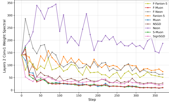
(c) Spectral norm of layer2.conv1
