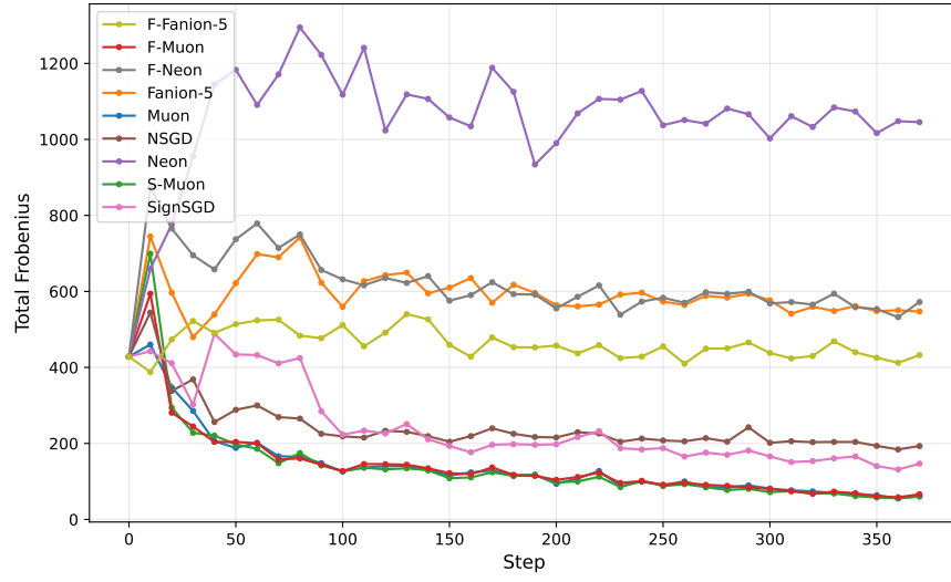
(a) Total Frobenius norm
