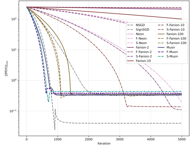
(b) The nuclear norm of the full gradient
