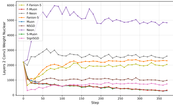
(e) Nuclear norm of layer2.conv1
