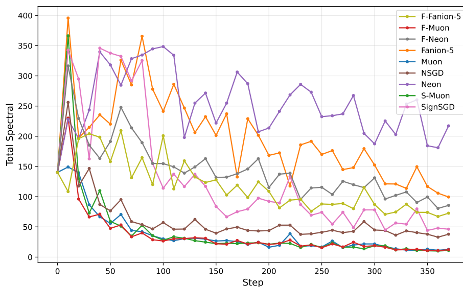
(b) Total spectral norm
