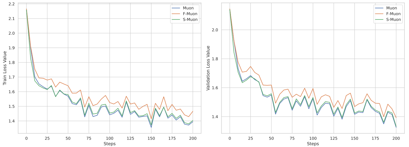
Рис. 7: Train and validation loss at the optimal learning rate for each optimizer.
