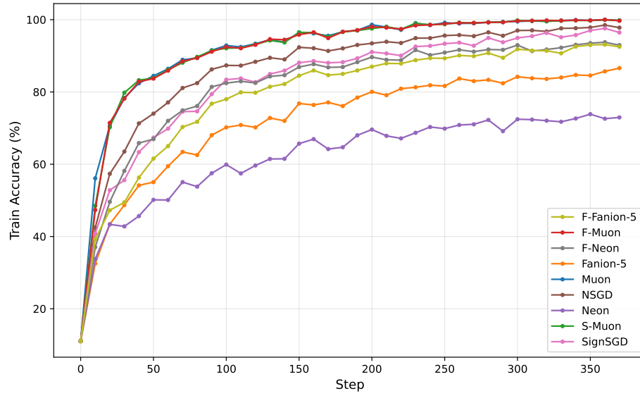
(a) Training accuracy
