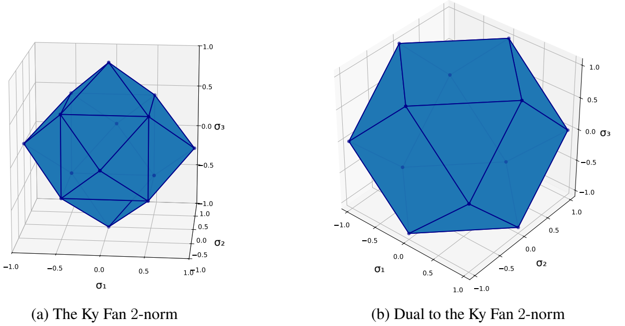
Рис. 9: Ky Fan 2-norm and its dual in the space of 3 singular values.
