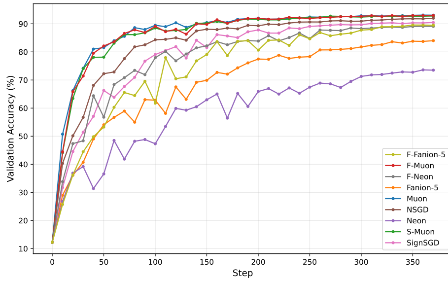
(b) Validation accuracy
