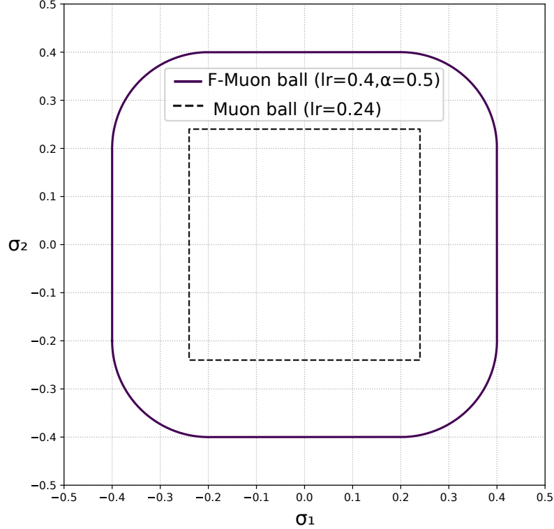
Рис. 3: The LMO balls of Muon and F-Muon for training a CNN on CIFAR-10.
