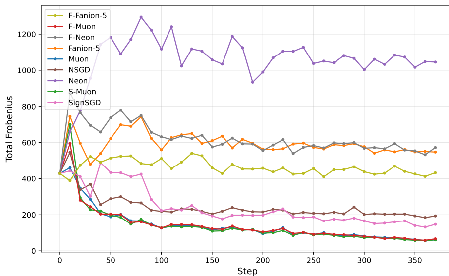
(a) Total Frobenius norm
