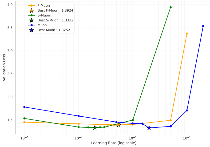
Рис. 6: Comparison of validation loss for Muon, F-Muon, and S-Muon across a range of learning rates. Stars denote the best learning rates for each optimizer. \alpha = 1/2 for F-Muon and S-Muon and \text{sign\_sgd\_coeff} = 1/3 for S-Muon.
