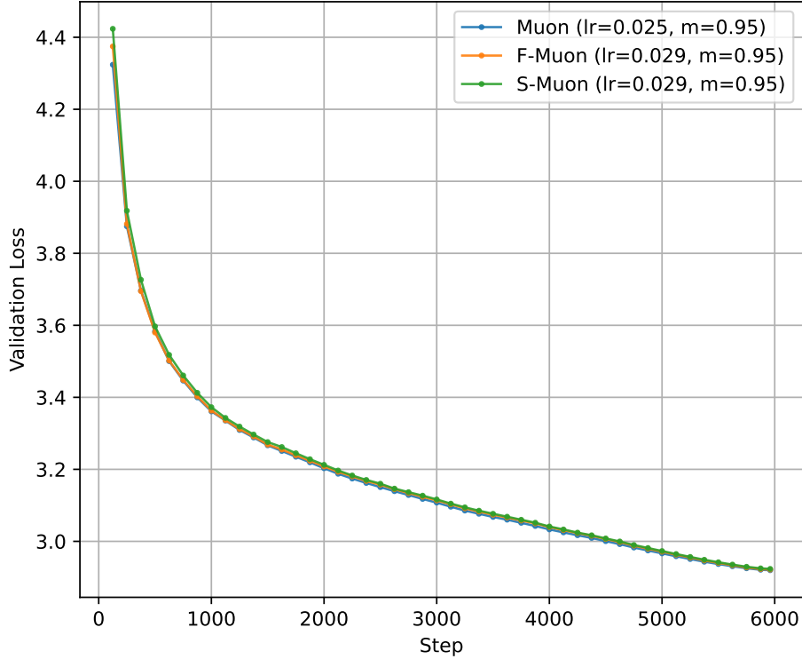
Рис. 5: The validation loss for GPT-2 Medium.
