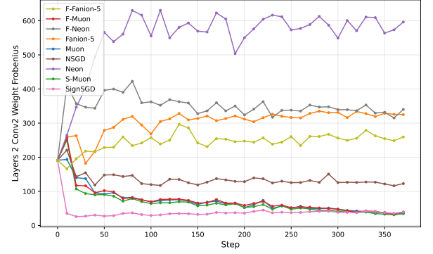
(b) Frobenius norm of layer2.conv2
