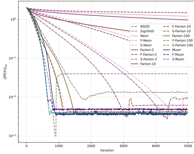
(a) The spectral norm of the full gradient
