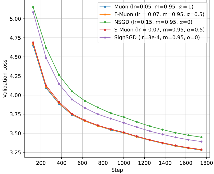
Рис. 4: The validation loss for NanoGPT.
