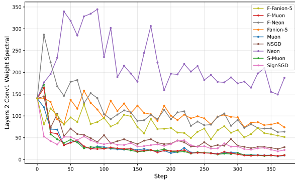
(c) Spectral norm of layer2.conv1
