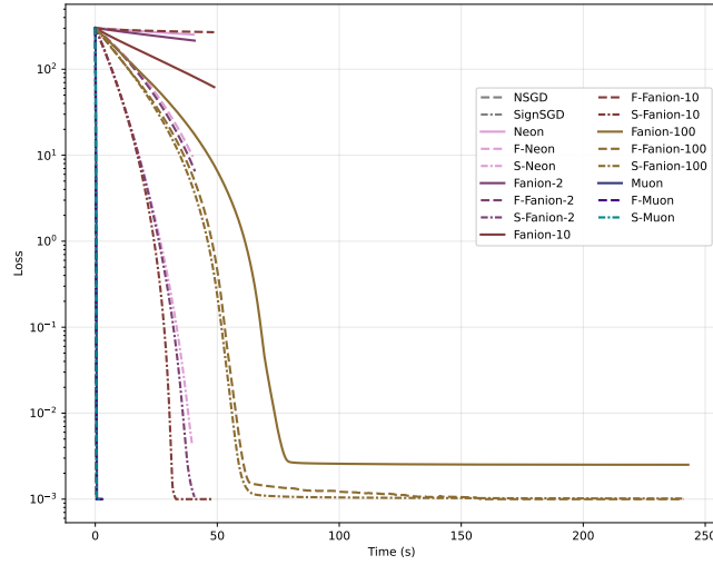
(c) The loss over time
