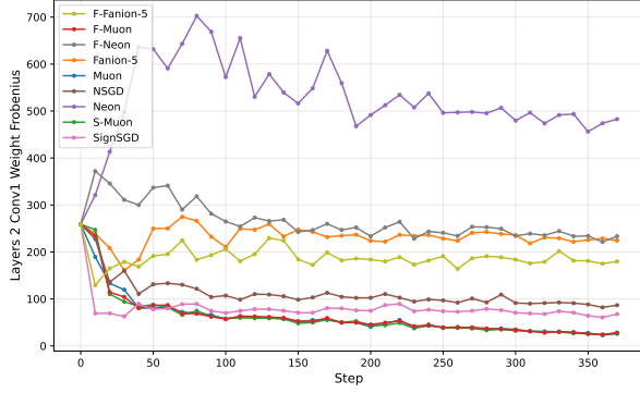
(a) Frobenius norm of layer2.conv1
