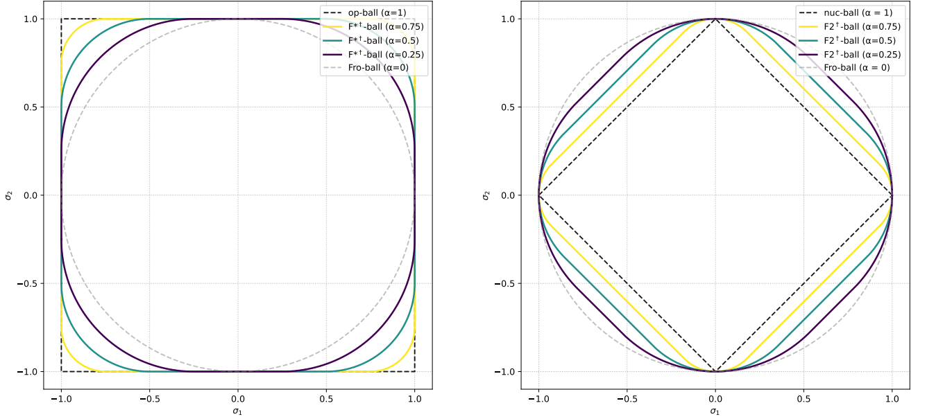
(a) lmo balls for F-Muon for different \alpha
