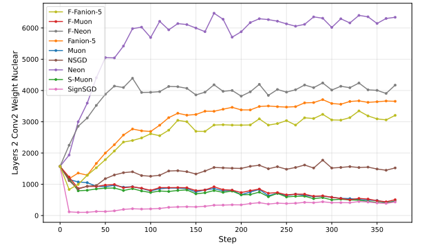
(f) Nuclear norm of layer2.conv2
