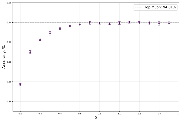
(a) With parameters tuned for Muon
