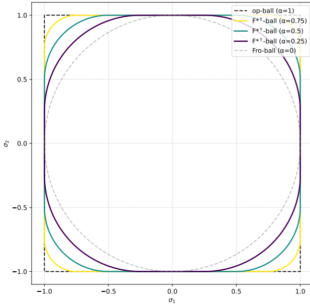
(a) Unit balls for F -Muon for different \alpha
