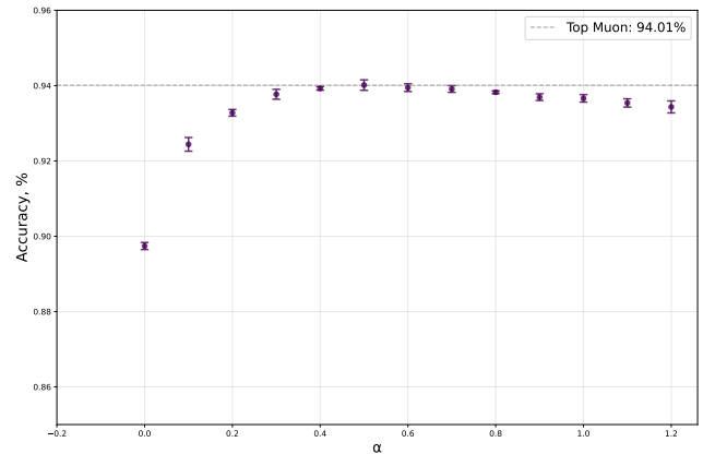
(b) With parameters tuned for F-Muon
