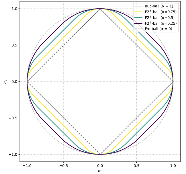
(b) Unit ball for F -Neon for different \alpha
