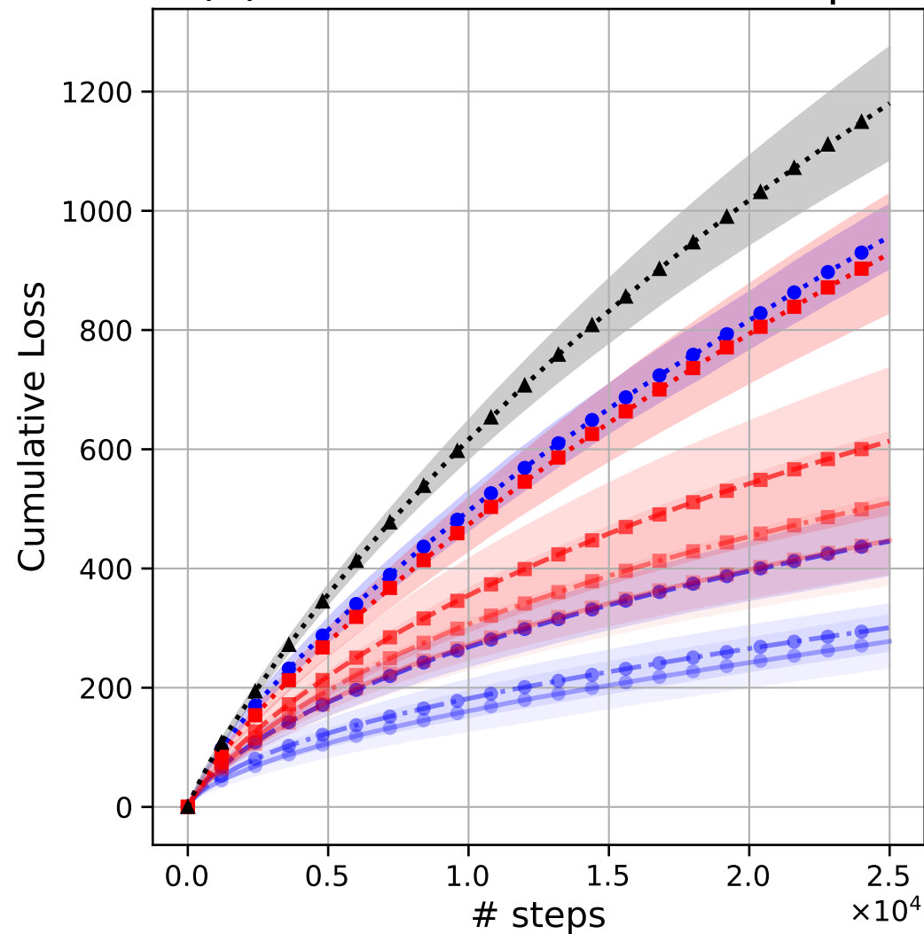
(a) Cumulative Loss vs Steps
