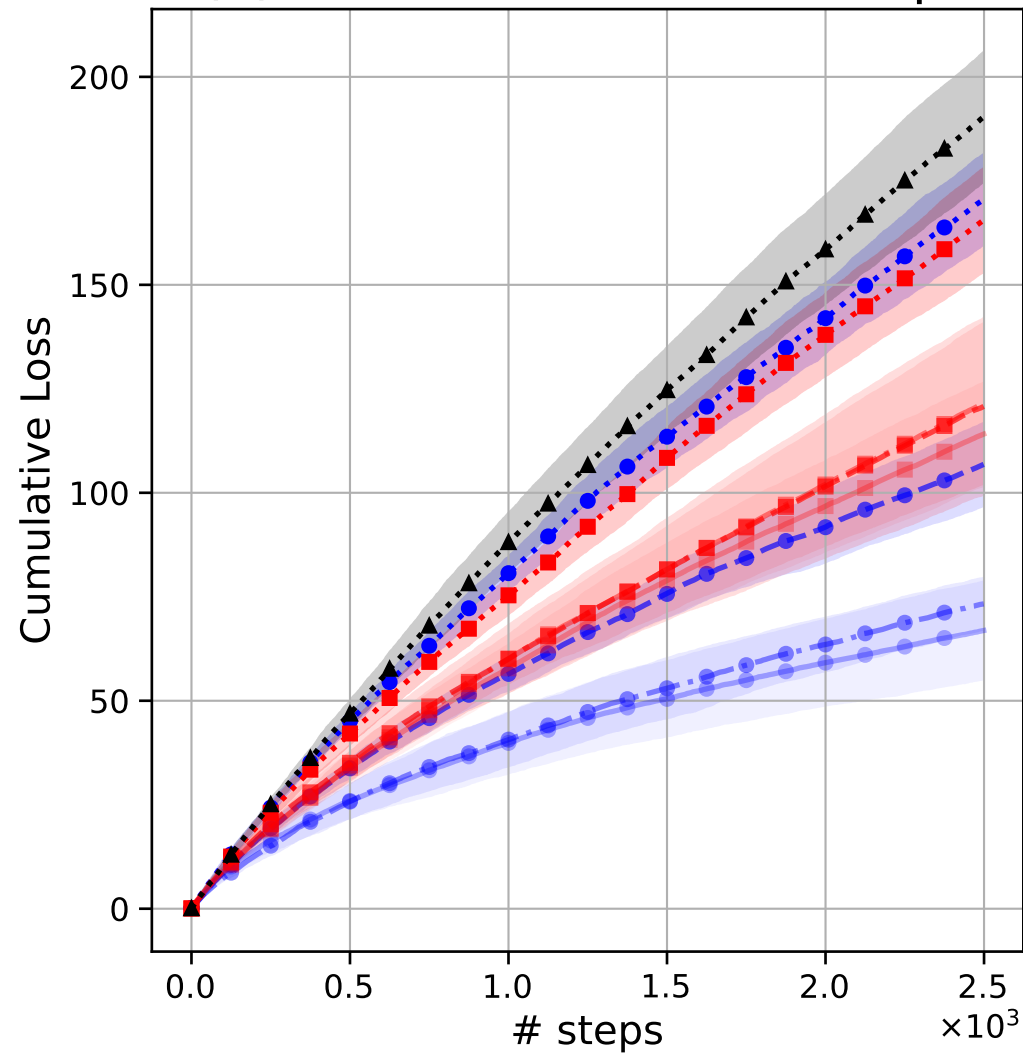
(a) Cumulative Loss vs Steps
