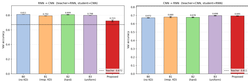
Baseline comparison — CIFAR-10 val accuracy (mean \pm std over 2 seeds)
