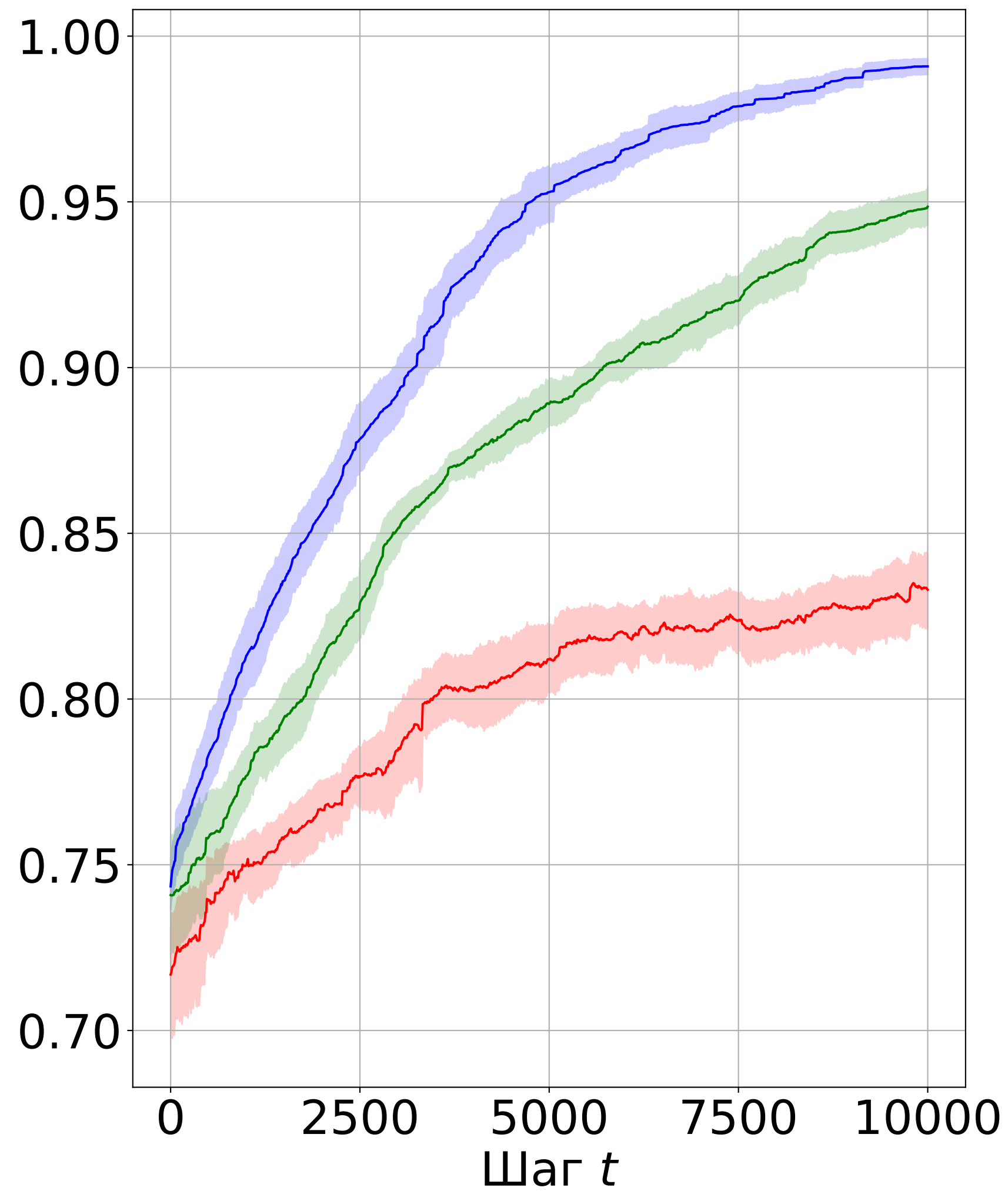
r2-score
