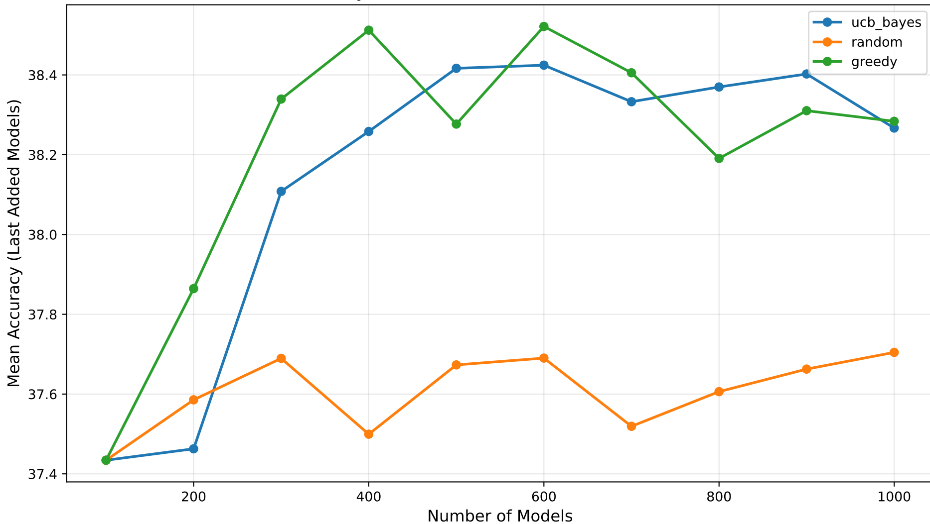
Mean Accuracy of Last Added Models vs Number of Models
