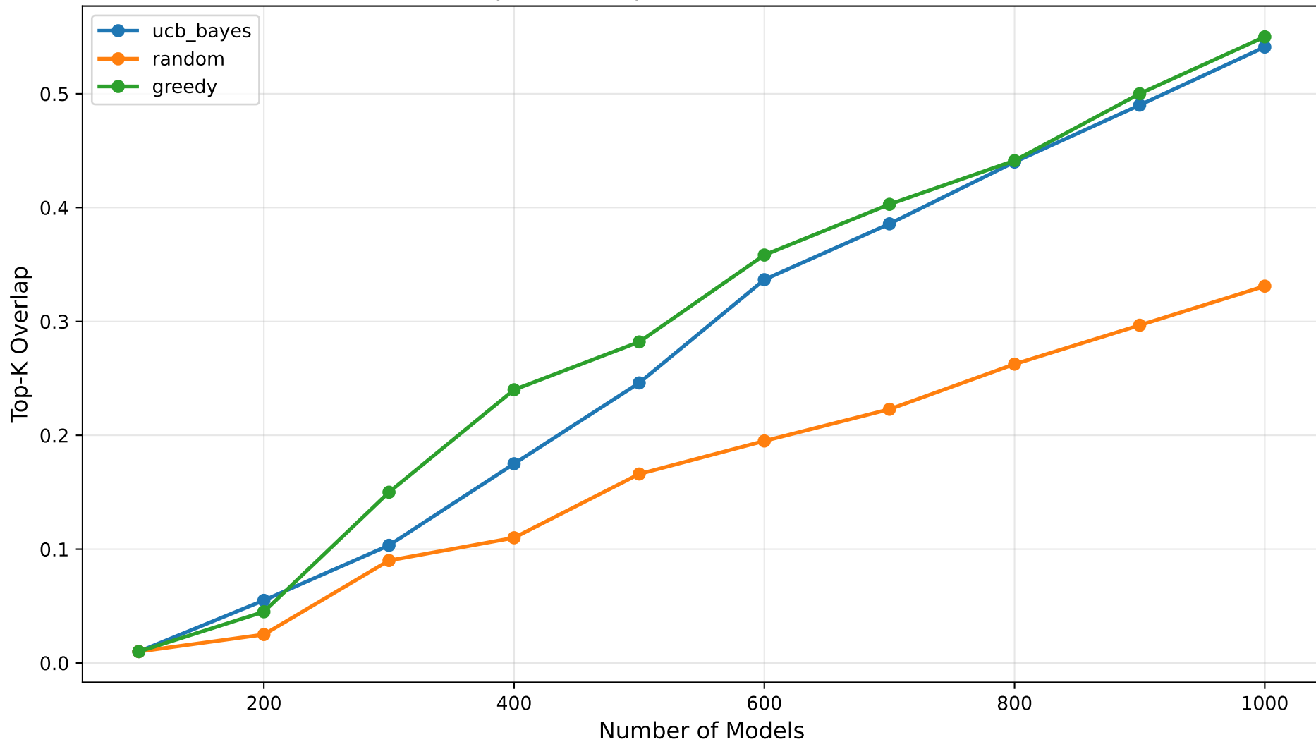
Top-K Overlap vs Number of Models
