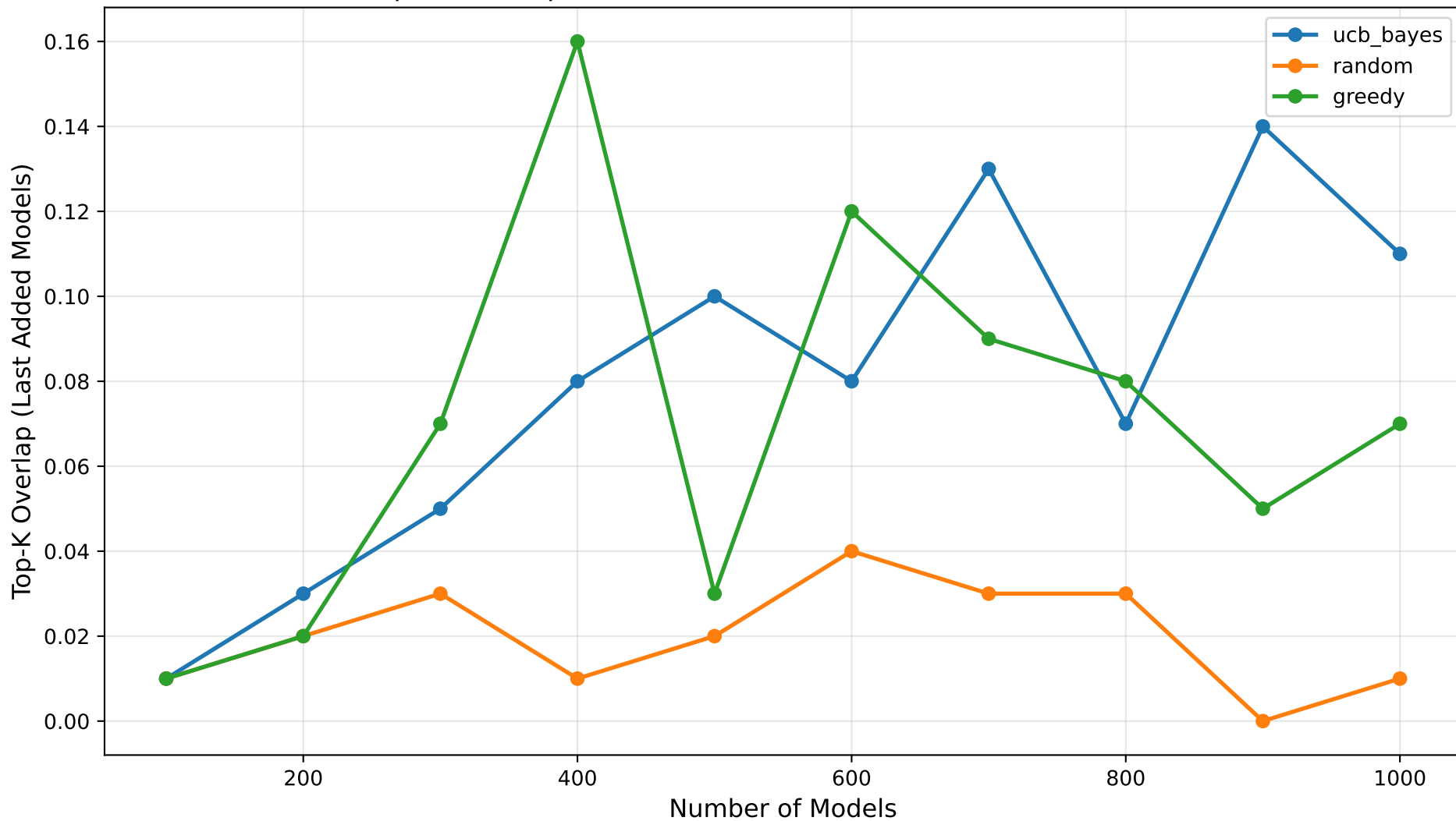
Top-K Overlap of Last Added Models vs Number of Models
