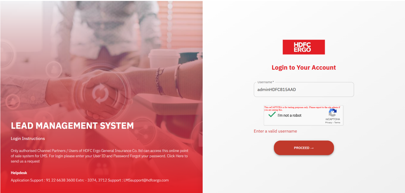
Screenshot: change_user_error.png
