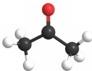
丙酮 ( \text{CH}_3 - \overset{\text{O}}{\underset{||}{\text{C}}} - \text{CH}_3 )
