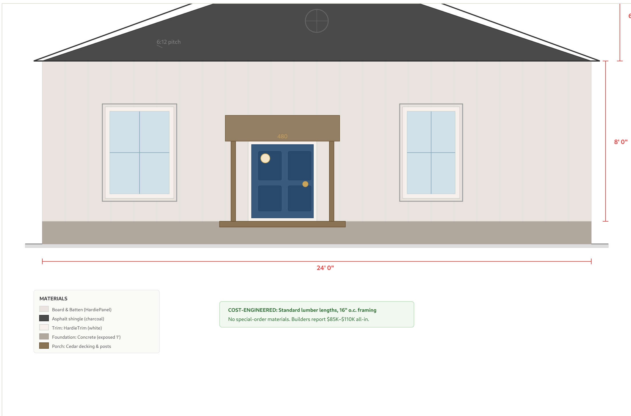
Fig. 2 — Front Elevation (South). Board & batten siding, gable roof 6:12, cedar porch.
