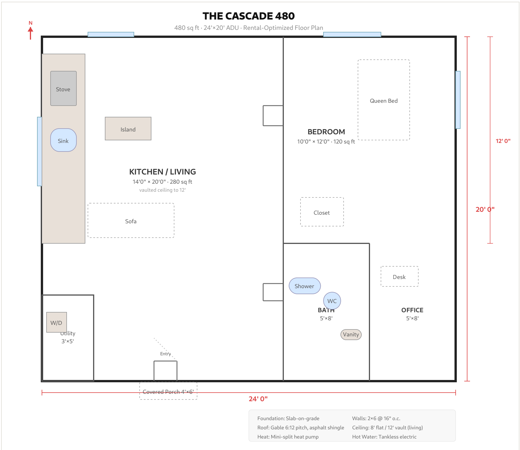
Fig. 1 — Floor Plan: 24'×20' ADU. Scale: 1/4" = 1'-0" when printed at 36"×24".
