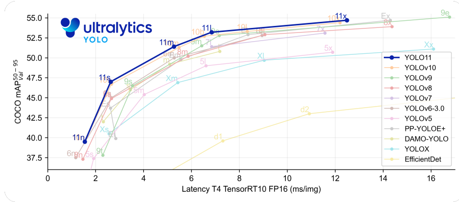
Figure 11: Performance Comparison Graph
