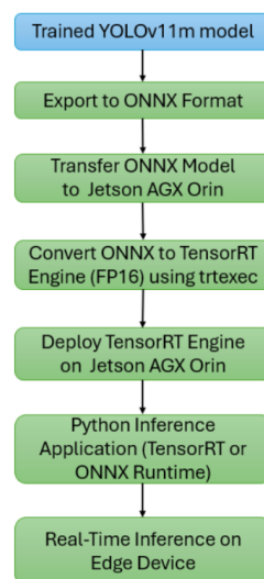
Figure 15: Model Deployment Pipeline Diagram
