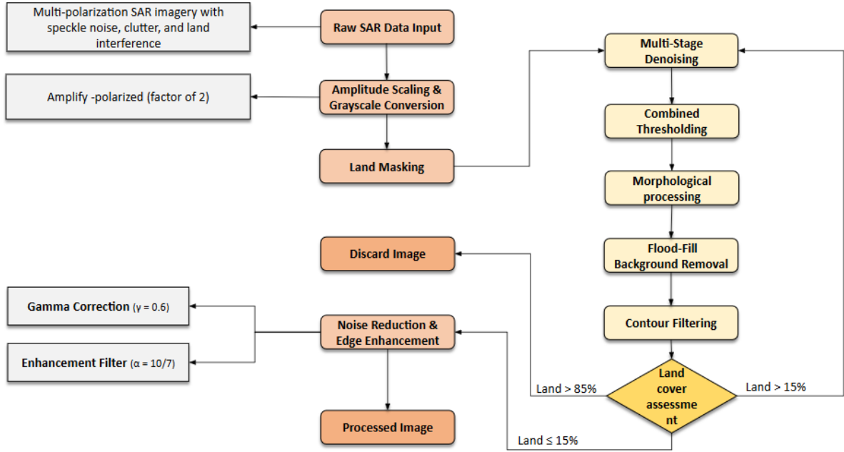
Figure 4: Preprocessing Subsystem Flowchart
