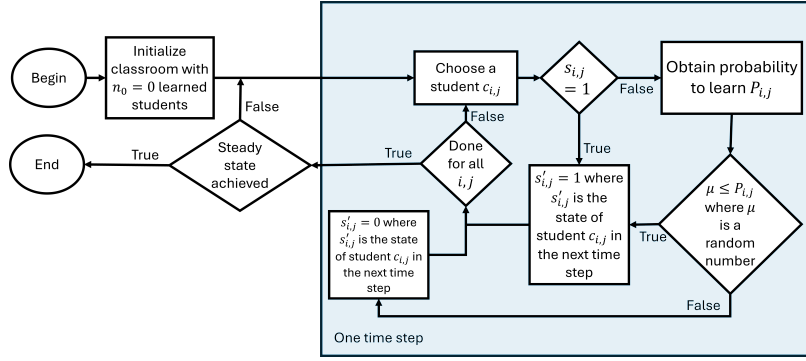
Figure 1: Flowchart for the pCA algorithm used in this work. The broadcast (TI) and nearest-neighbor (PI) regimes differ in how the update probability P_{i,j} is determined, as described in the text.
