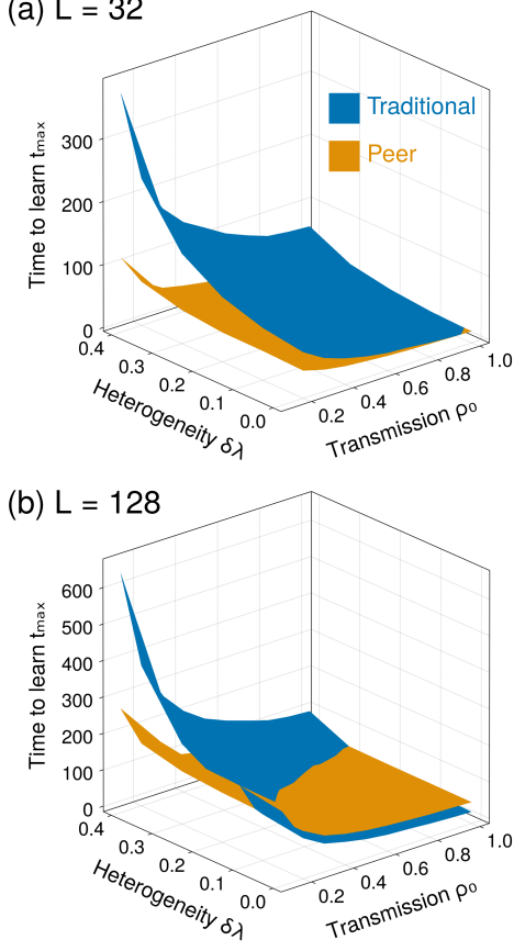
FIG. 5. Time to learn t_{\max} as a function of positional learning factor \rho_0 and heterogeneity \delta\lambda of PI (inner corner SA) and TI for two different class sizes N = L^2 ((a) L = 32 and (b) L = 128 ). The blue surface represent TI and the orange surface represents PI. Lower time to learn indicates better learning.
