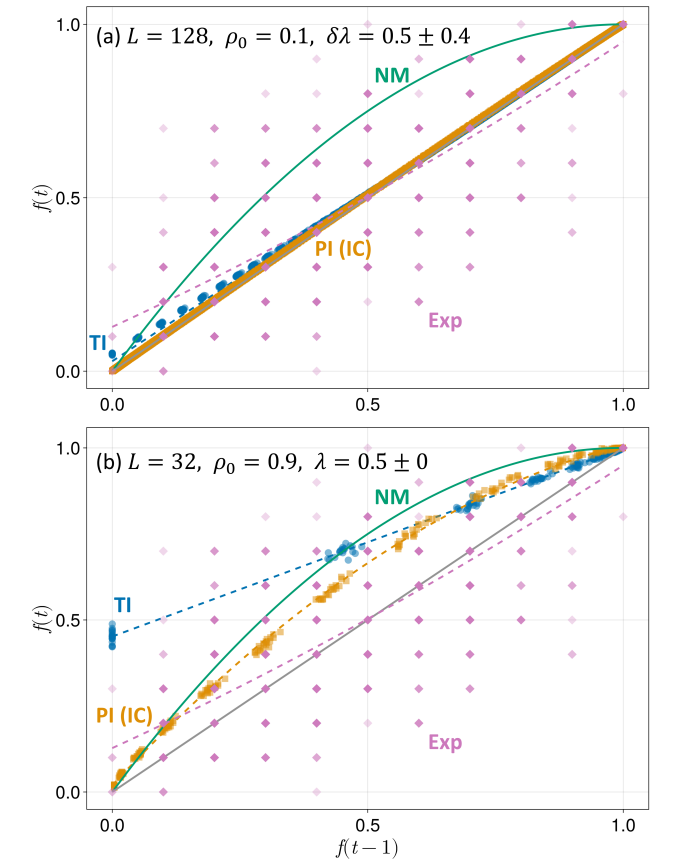
FIG. 6. Return map for selected parameter sets for both TI and PI. Blue circles represent the data points for TI and orange squares represent the data points for PI. Pink diamonds represent data points from Roxas' work [11] for comparison. The darker data points mean that more points overlap on those coordinates. The corresponding best-fit quadratic function obtained using the Levenberg-Marquardt algorithm for each set of data points are shown in dashed lines in their corresponding color and are discussed in the text. The green line represents Nitta's theoretical model (Equation 2) and the gray line represents y = x .
