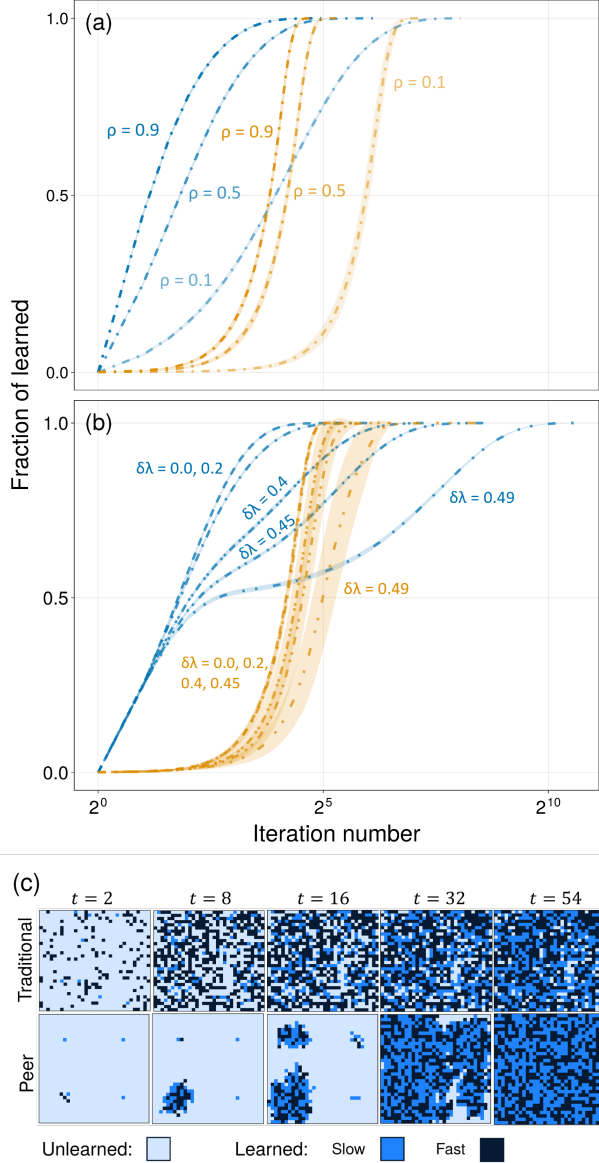
FIG. 4. Different monotonic increase of the total fraction of students in the learned state over iteration number. The blue line represents the TI mode while the orange line represents the PI mode. Unless indicated, the parameters are fixed such that N = 64 , \rho_0 = 0.5 , \delta\lambda = 0.2 (fairly homogenous) and an Inner Corner SA for PI mode. (a) Plots for varied \rho_0 -values, introducing varying degrees of shifts along the iteration (time) axis. (b) Plots for varied \delta\lambda -values. (c) Representative development of classroom spatial configuration ( L = 32 , \rho_0 = 0.3 ) observed for different iteration numbers from t = 2 (each column doubles the previous t ) for TI (first row) and PI (second row) modes. The learned and unlearned states are differentiated by the color intensity, with \lambda = 0.9 (darker) and 0.1 (lighter) shades.
