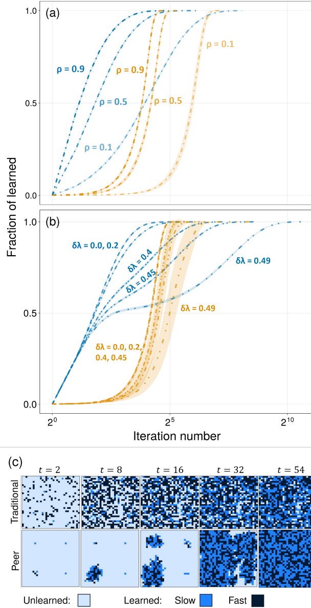
Figure 4: Monotonic increase of the learned agent fraction over iteration number for both interaction regimes. Blue lines represent the broadcast (TI) regime and orange lines represent the nearest-neighbor (PI) regime with inner corner seating arrangement. Bands represent the min-max range across 20 independent randomized runs. Fixed parameters unless otherwise indicated: N = 64 , \rho_0 = 0.5 , \delta\lambda = 0.2 , inner corner SA for the nearest-neighbor regime. (a) Effect of coupling strength \rho_0 . (b) Effect of heterogeneity parameter \delta\lambda . (c) Representative spatial configurations of the lattice ( L = 32 , \rho_0 = 0.3 ) at successive iteration numbers (each column doubles the previous t , starting from t = 2 ) for the broadcast regime (top row) and nearest-neighbor regime (bottom row). Color intensity encodes agent learning rate, with darker shades indicating higher \lambda values.
