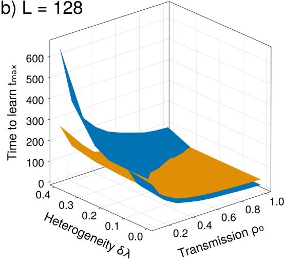
Figure 5: Total relaxation time t_{\max} as a function of coupling strength \rho_0 and heterogeneity \delta\lambda for the broadcast (blue surface) and nearest-neighbor (orange surface) regimes, for two system sizes: (a) N = 32^2 and (b) N = 128^2 . The nearest-neighbor regime uses the inner corner seating arrangement. Lower t_{\max} indicates faster collective relaxation.
