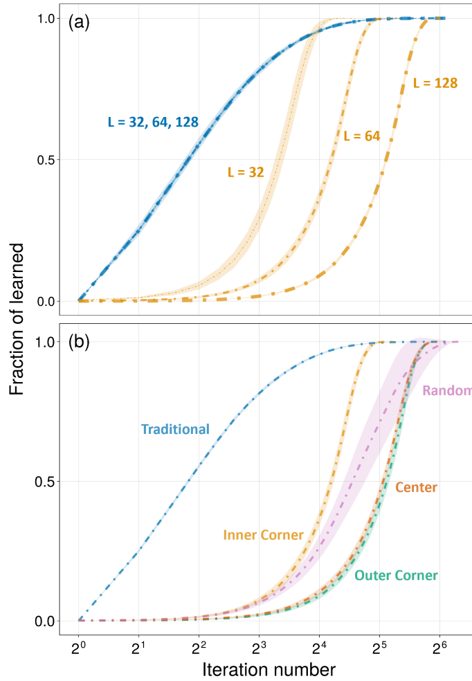
Figure 3: Monotonic increase of the learned agent fraction over iteration number for both interaction regimes. Blue corresponds to the broadcast (TI) regime; all other colors correspond to the nearest-neighbor (PI) regime with different seating arrangements (SAs): yellow-orange (inner corner), orange (center), green (outer corner), and pink (random). Line width is proportional to system size N . Bands represent the min-max range across 20 independent randomized runs. Fixed parameters: \rho_0 = 0.5 , \delta\lambda = 0.2 . (a) Effect of system size N ; the inner corner SA is used for the nearest-neighbor regime. (b) Effect of seating arrangement for a fixed system size.
