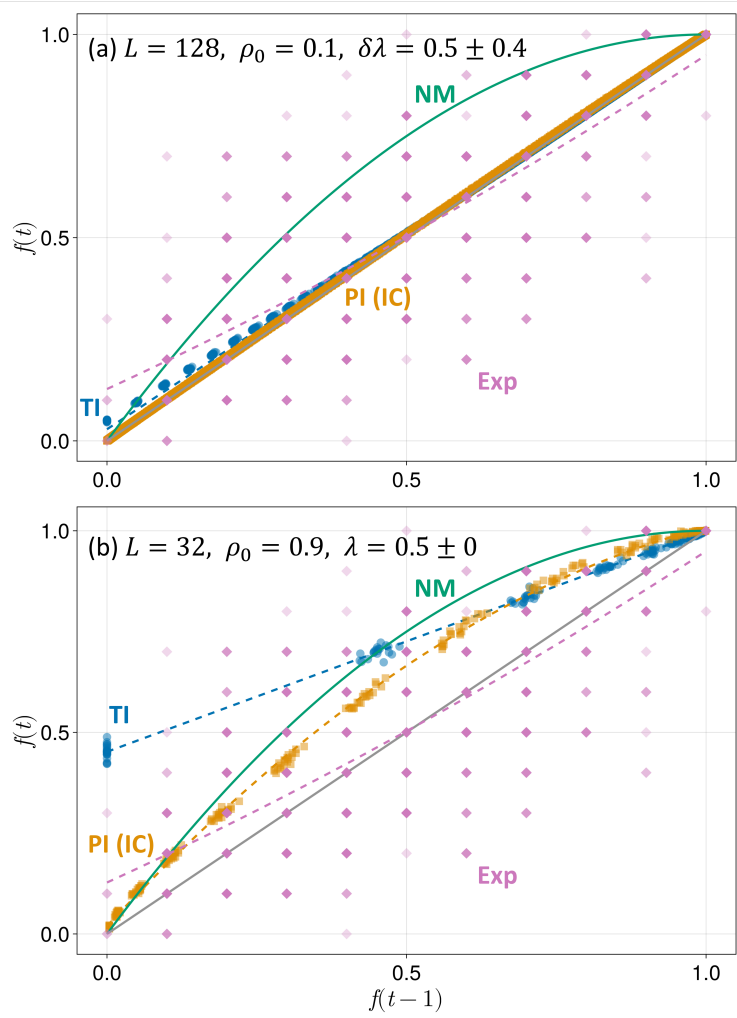
Figure 6: Return map of the learned agent fraction f_t against f_{t-1} for selected parameter sets. Blue circles represent broadcast (TI) regime data points; orange squares represent nearest-neighbor (PI) regime data points; pink diamonds represent empirical data from Roxas (co-author). Darker points indicate higher overlap of data points at those coordinates. Dashed lines show the best-fit functions obtained using the Levenberg-Marquardt algorithm for each dataset. The green line represents the theoretical prediction of Nitta (2019) and the gray line represents y = x . (a) Large system size N = 128^2 . (b) Small system size N = 32^2 .
