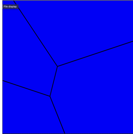
Figure 1: Voronoi diagram computed from four sites using linear enumeration and Sutherland–Hodgman clipping.
