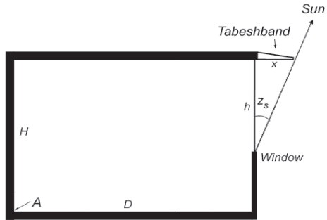
Summer solstice
