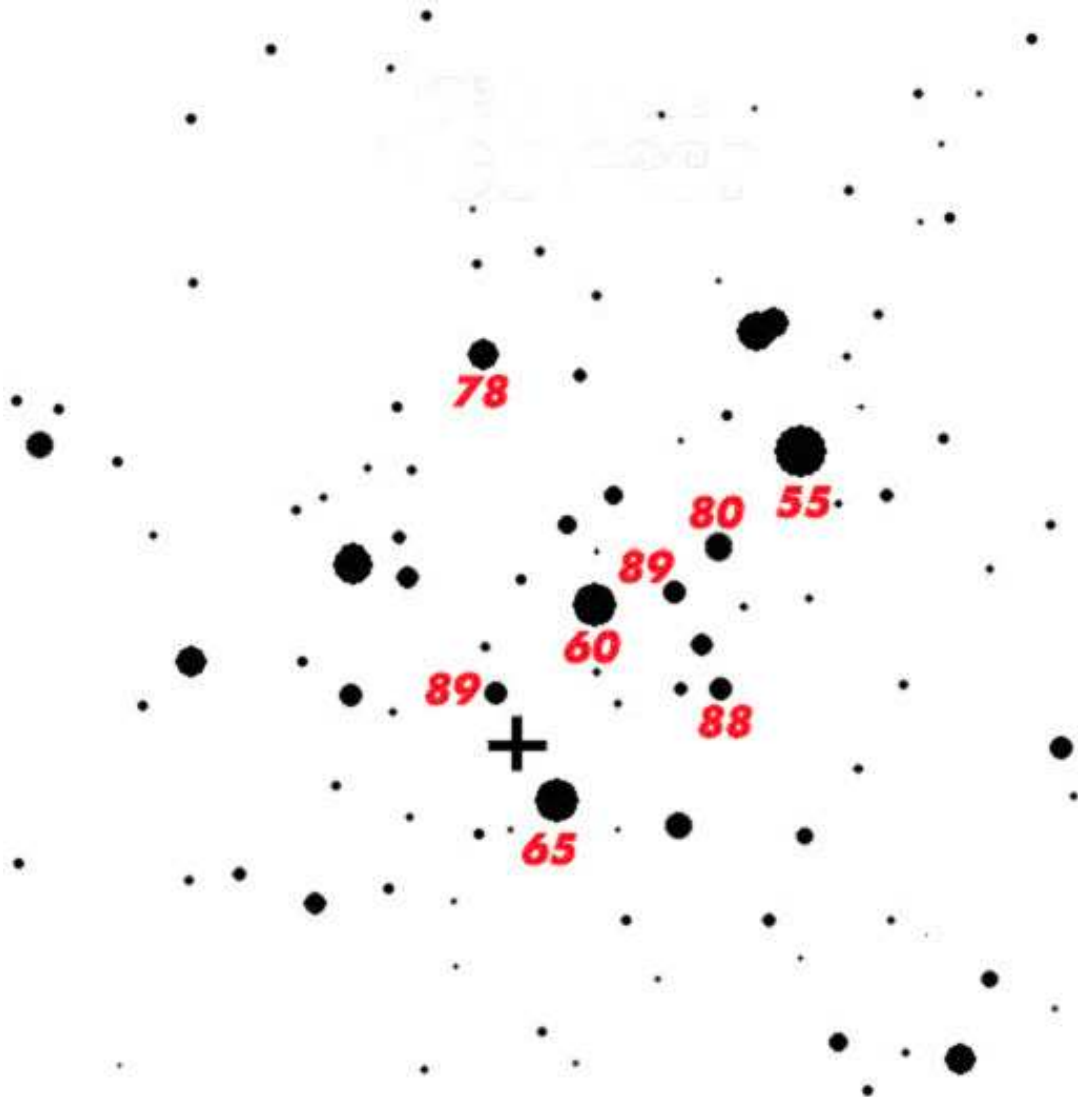
Chart 2 – NGC 6231
