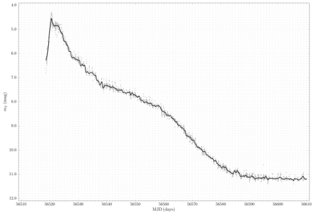
Nova Del 2013 – Johnson V light curve
