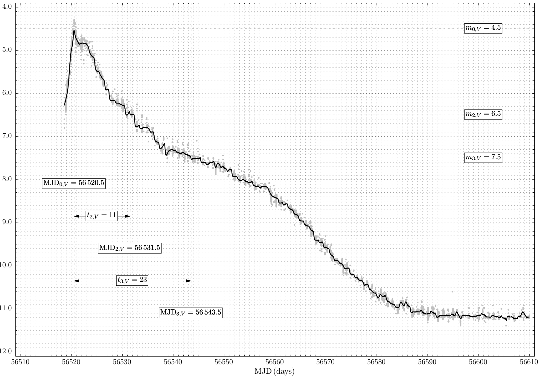
Nova Del 2013 – Johnson V light curve
