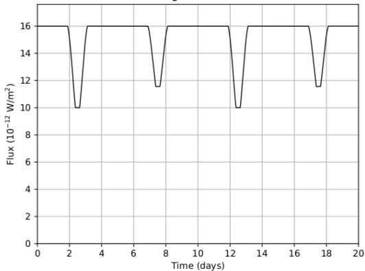
Light curve A
