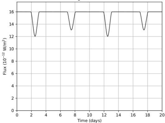
Light curve B
