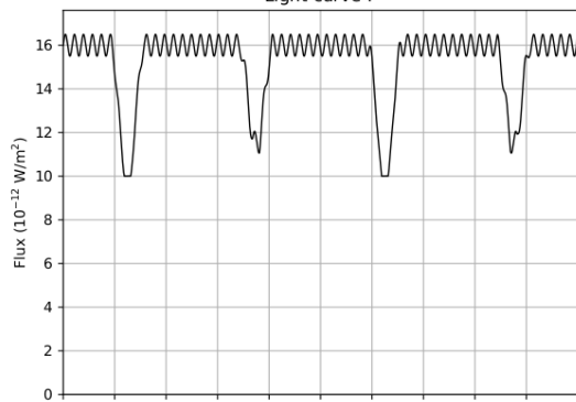
Light curve F
