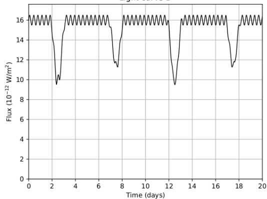
Light curve D
