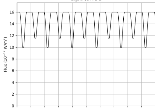
Light curve E
