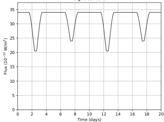
Light curve C
