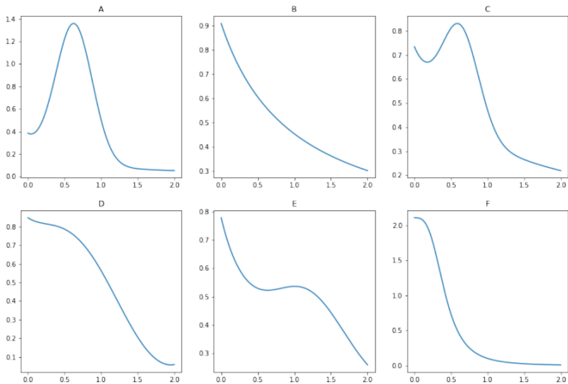
Figure 1: Probability density of all possible galaxy pairs
