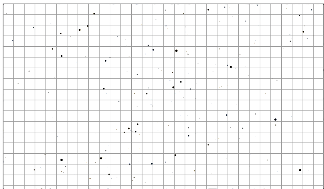
Initial
