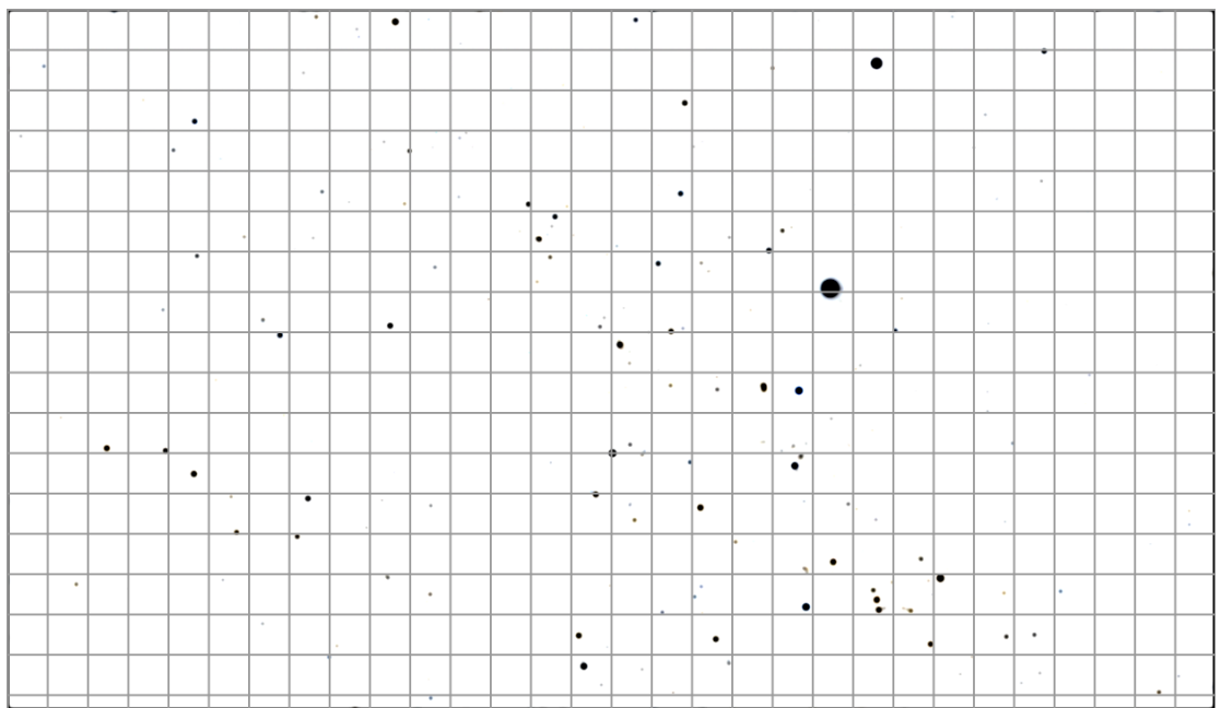
Final
