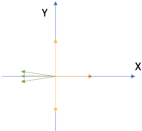
Rest Frame
