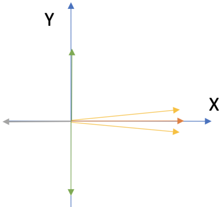
Lab Frame
