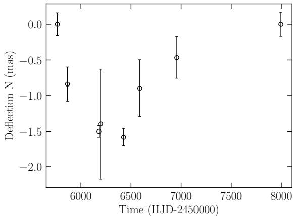
Figure 8: These figures show the astrometric deflection in East and North directions induced by the black hole. (Students are not required to make these plots.)
