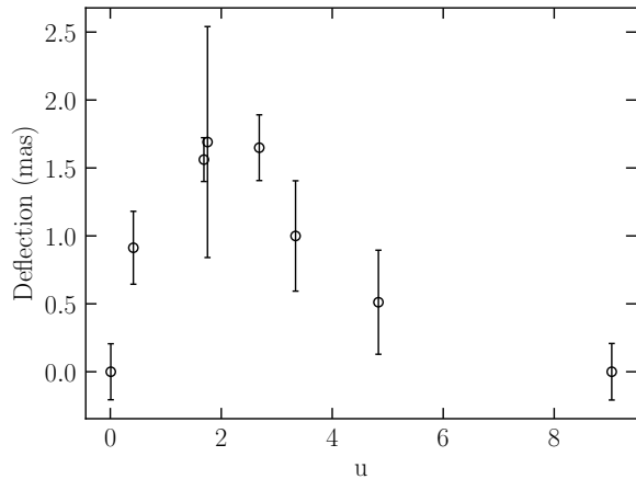
Figure 9: Total astrometric deflection as a function of u . Students are asked to make this plot in part (f).
