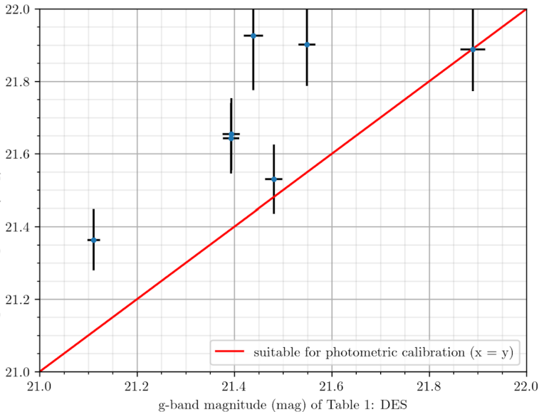
g-band magnitude (mag) of Table 2: SDSS
