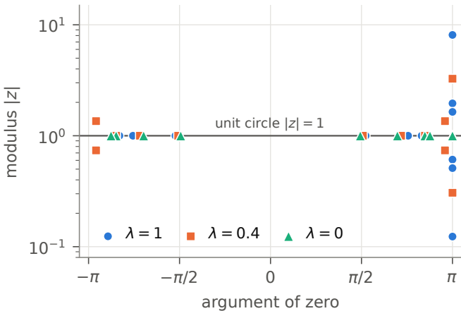
(a) Zeros of Z_\lambda
