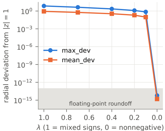
(b) Distance from the circle
