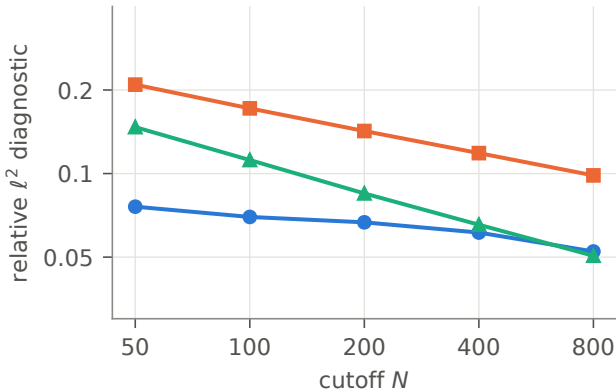
(a) \Re(s) > 1 , one-sided completion
