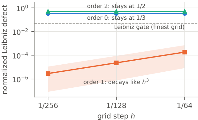
(a) Leibniz defect under refinement
