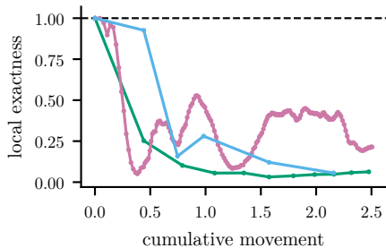
(a) r13, seed 0
