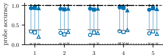
(e) r8 / r10 law TV
