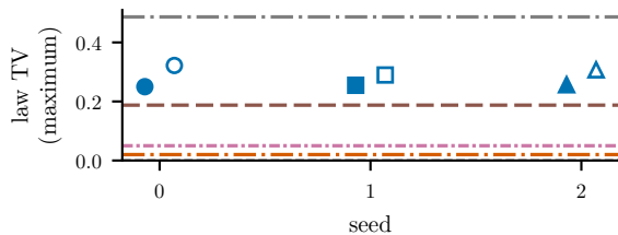
(e) r8 / r10 law TV
