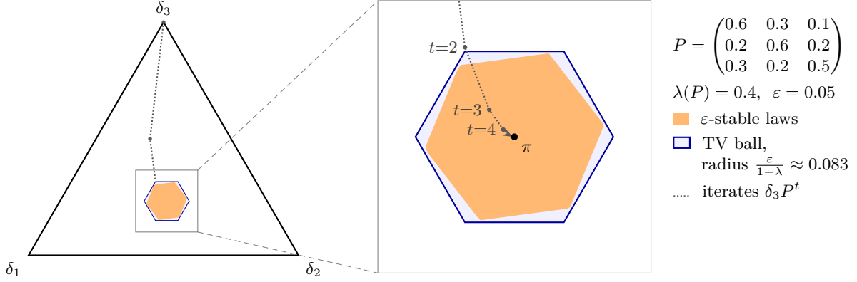
Figure 4. Contractive objecthood on three states. Left: the simplex \Delta(\{1, 2, 3\}) ; the boxed region is enlarged on the right. The set of \varepsilon -stable laws (orange, computed on a fine grid) lies inside the total variation ball of radius \varepsilon/(1 - \lambda) around the stationary law \pi guaranteed by Corollary 7.1; in the plane of the simplex this ball is a hexagon. Any two orange laws are therefore within 2\varepsilon/(1 - \lambda) \approx 0.17 of each other, as Theorem 3.6 asserts. The dotted path shows the iterates \delta_3 P^t converging geometrically to \pi (Proposition 7.1).
