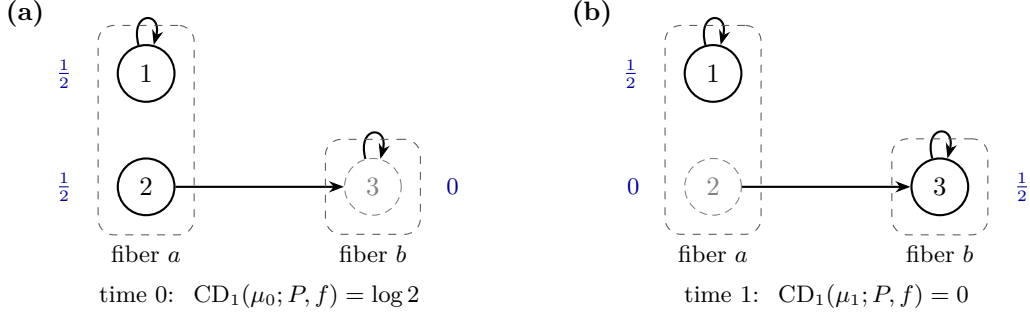
Figure 3. The closure deficit depends on the current law (Example 6.1). Microstates 1 and 2 form macrostate a , and state 3 forms macrostate b ; current masses are shown in blue, and states of zero mass are dashed. (a) At time 0 both microstates in fiber a have mass 1/2 , but 1 stays in a while 2 moves to b , so the macrostate does not determine the macroscopic future and CD_1 = \log 2 . (b) One step later state 2 has mass zero, every positive-mass fiber has a single macroscopic future, and CD_1 = 0 .
