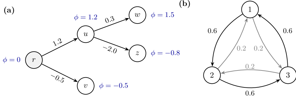
Figure 2. (a) On a tree every antisymmetric edge field is a gradient. Edge labels give a(\text{parent}, \text{child}) ; summing them along the unique path from the root r gives the potential \phi (blue), and a(u, v) = \phi(v) - \phi(u) on every edge. (b) A driven three-state ring, with holding probability 0.2 at each state. Each log-ratio equals \log 3 , so the cycle affinity is 3 \log 3 and the field is not a gradient. Deleting any one edge of the ring leaves a tree, on which the restricted field is a gradient.
