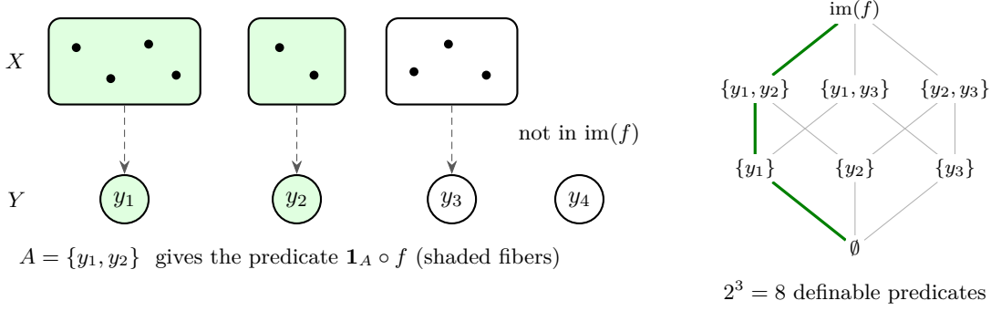
Figure 5. Definable predicates of a lens with |\text{im}(f)| = 3 . Left: a predicate definable through f is constant on fibers, so it is determined by the set A \subseteq \text{im}(f) of images on which it equals one; values of g off the image, such as at y_4 , are irrelevant. Right: the 8 definable predicates ordered pointwise form the lattice of subsets of \text{im}(f) . A strictly increasing chain, such as the highlighted one, has at most |\text{im}(f)| + 1 = 4 elements.
