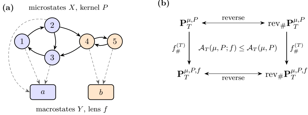
Figure 1. The setting. (a) A finite Markov chain on microstates is observed through a lens f that merges microstates into macrostates; the observed process is f(X_t) . (b) Reversing paths and applying the lens commute (Lemma 4.2). The arrow is the divergence between the top row of laws, and the observed arrow the divergence between the bottom row, so the data-processing inequality yields Theorem 3.1.
