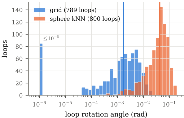
(a) canonical learned metrics (medians marked)
