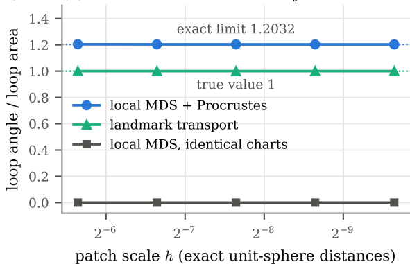
(b) area-normalised holonomy under refinement
