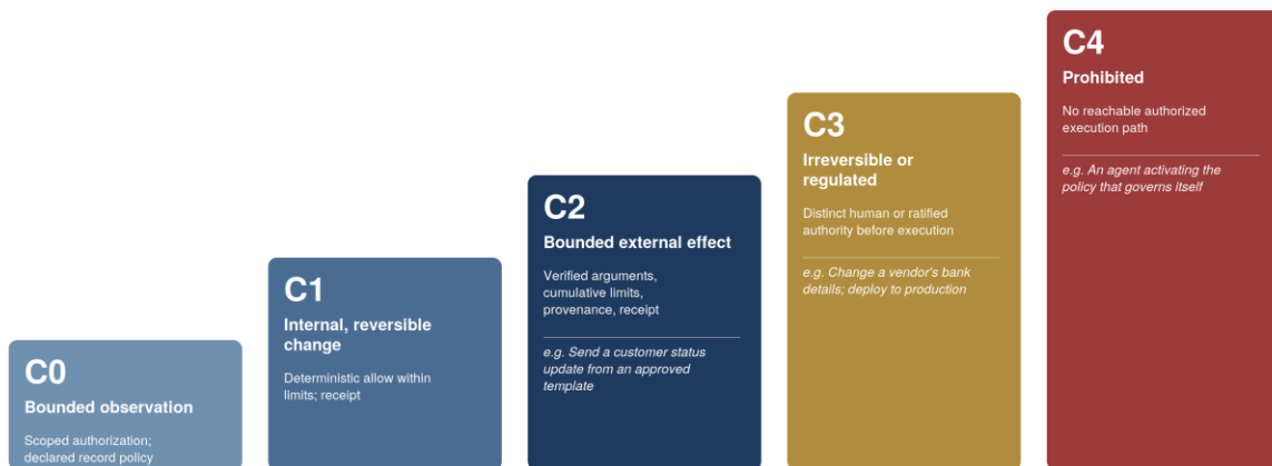
Figure 5. Consequence classes C0 to C4 and their default control postures. The class is computed from the approved manifest and verified context, never from the agent's description.
