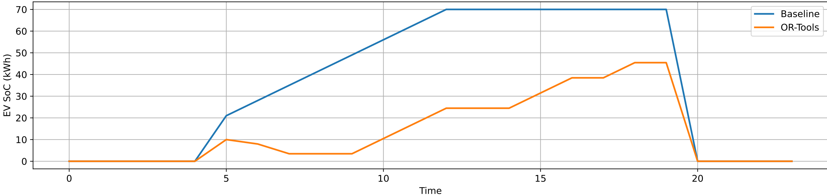
Electric Vehicle State of Charge
