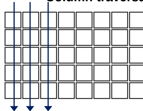
Column traversal
