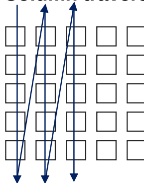
Column traversal
