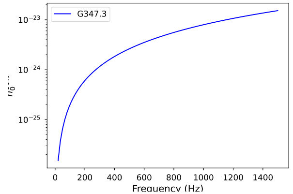
Figure 7. 90% confidence upper limits on the gravitational wave amplitude h_0 for G347.3.
