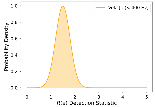
Figure 2. R(a) detection statistic distribution for the Vela Jr. searches below 400 Hz.
