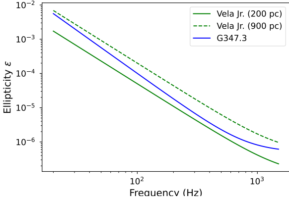
Figure 8. Strict upper limits on the equatorial ellipticity \epsilon .
