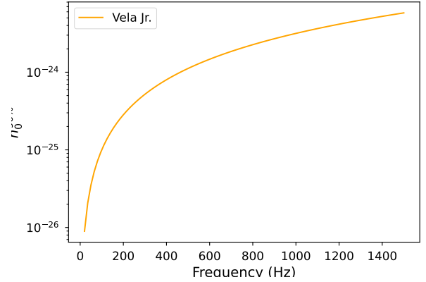
Figure 6. 90% confidence upper limits on the gravitational wave amplitude h_0 for Vela Jr.
