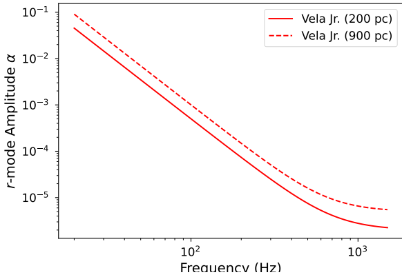
Figure 9. Strict upper limits on the r -mode amplitude \alpha .
