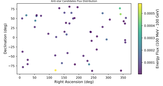
Figure 11. Positions and energy flux limits for Anti-star candidates in the 100 MeV - 100 GeV range.
