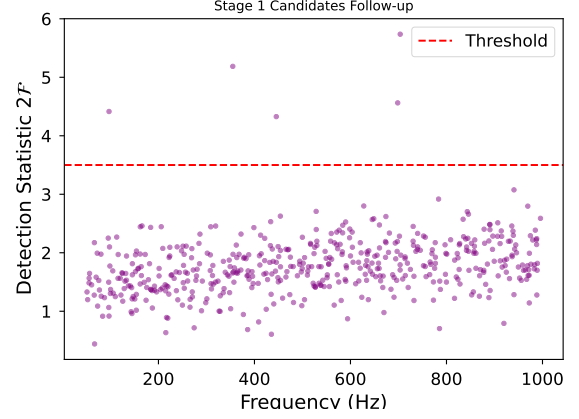
Figure 5. Approximation of the scattered frequency versus 2\mathcal{F} detection statistic.
