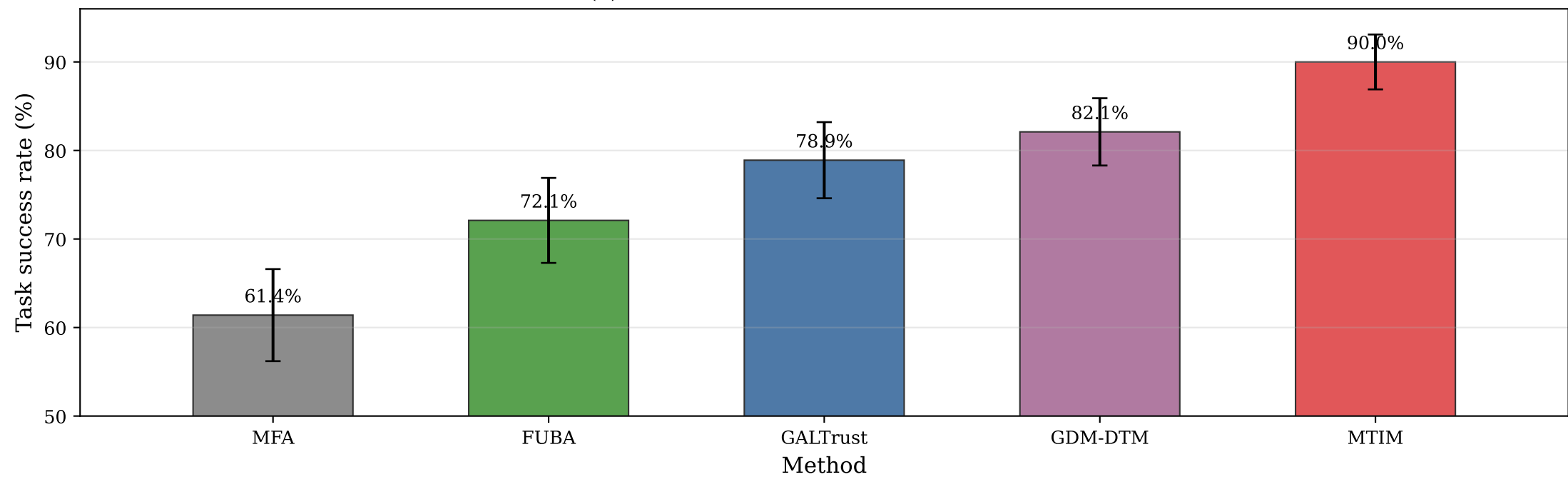
(c) Task success at 30% malicious ratio
