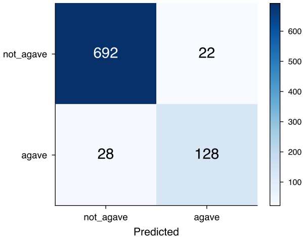
v11 confusion · threshold 0.60
