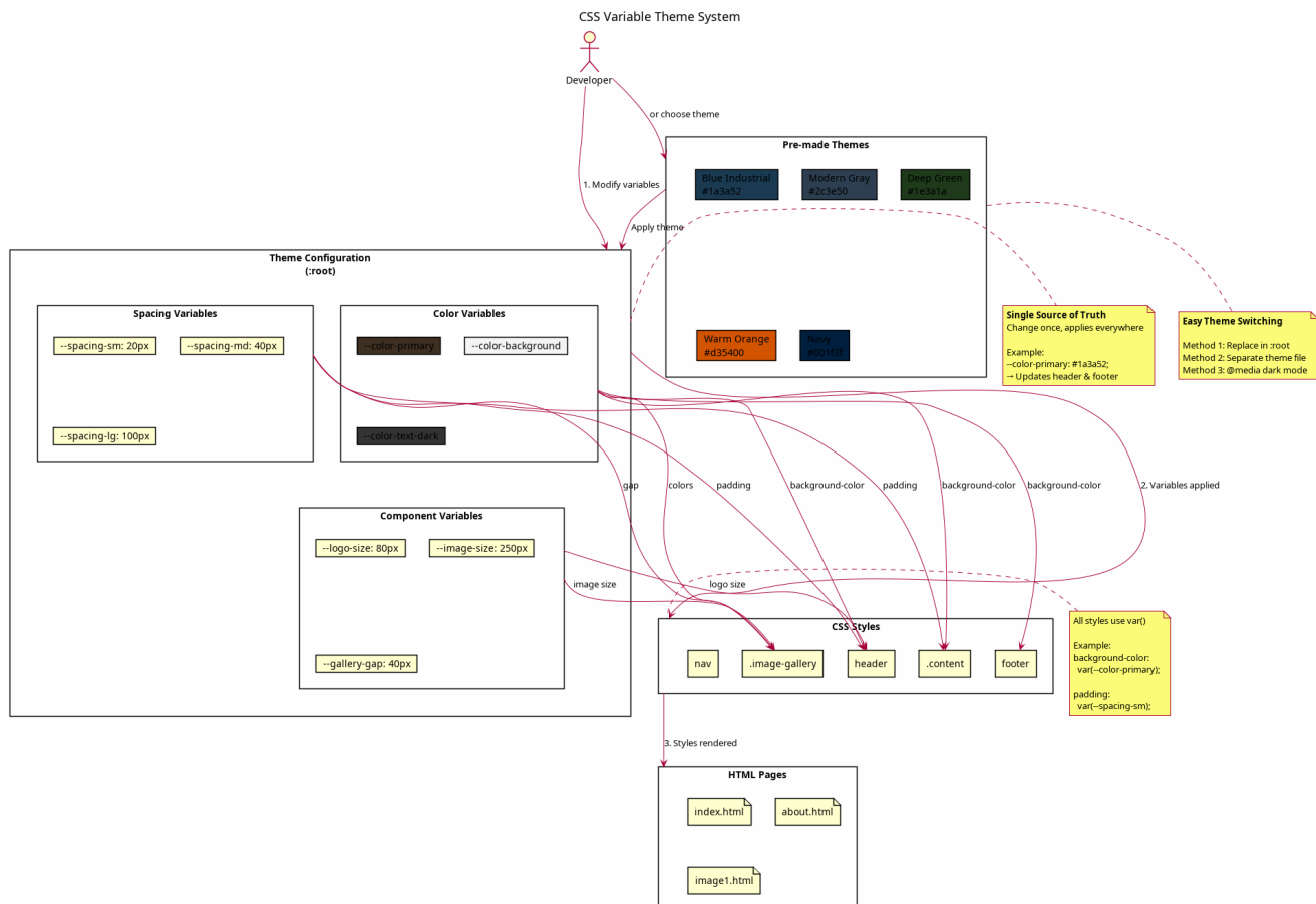
Figure 5. Theme System
