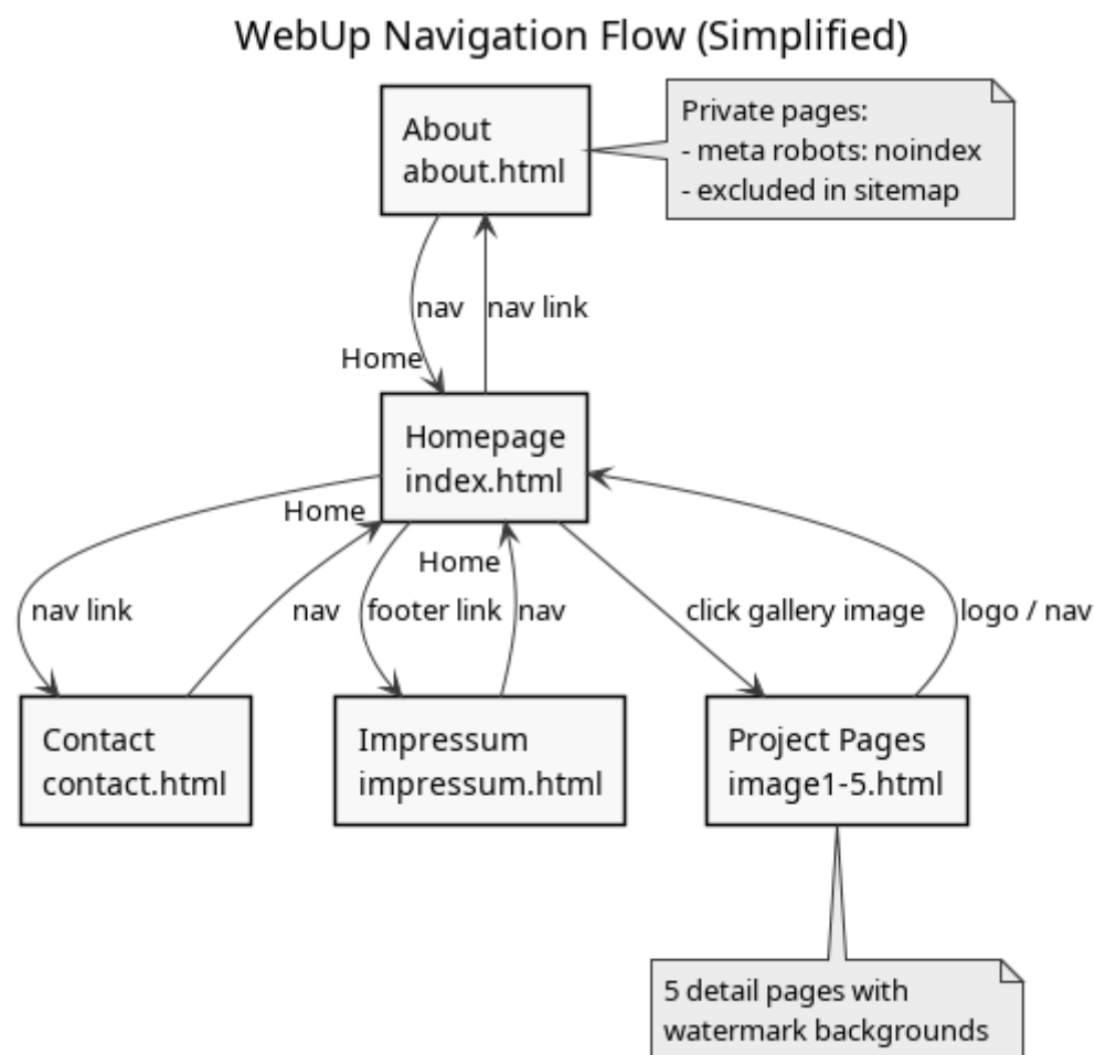
Figure 3. Navigation Flow
