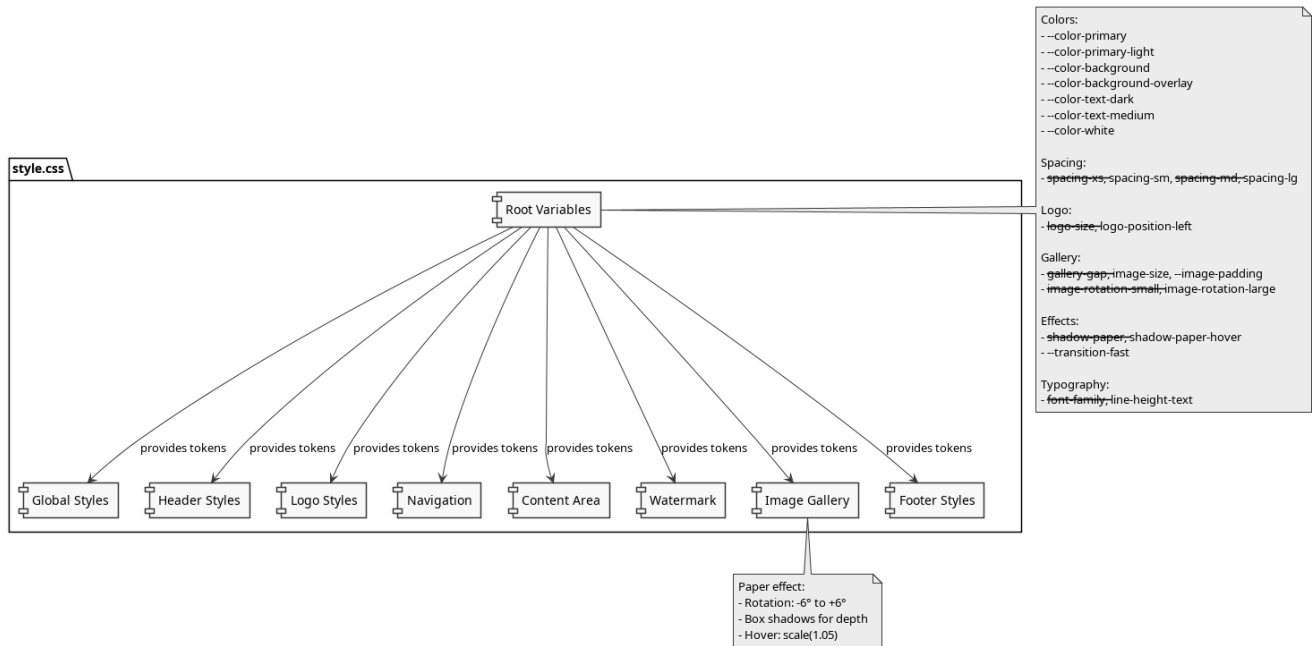
Figure 4. CSS Architecture
