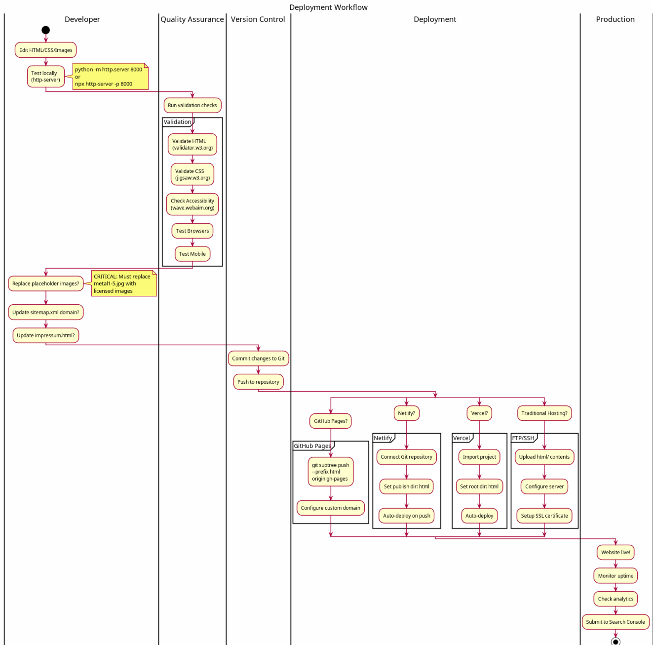
Figure 7. Deployment Workflow
