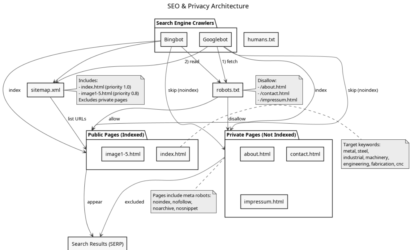
Figure 6. SEO & Privacy Architecture
