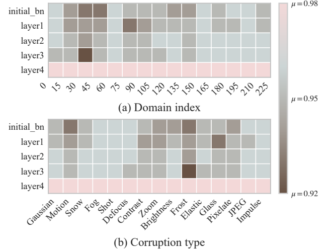
Fig. 9: Per-layer retention gates \mu_t^l of CLR on ImageNet-C (ResNet-50) . (a) Gates over the long-horizon T-CS stream. (b) Gates per corruption type under T-CS.
