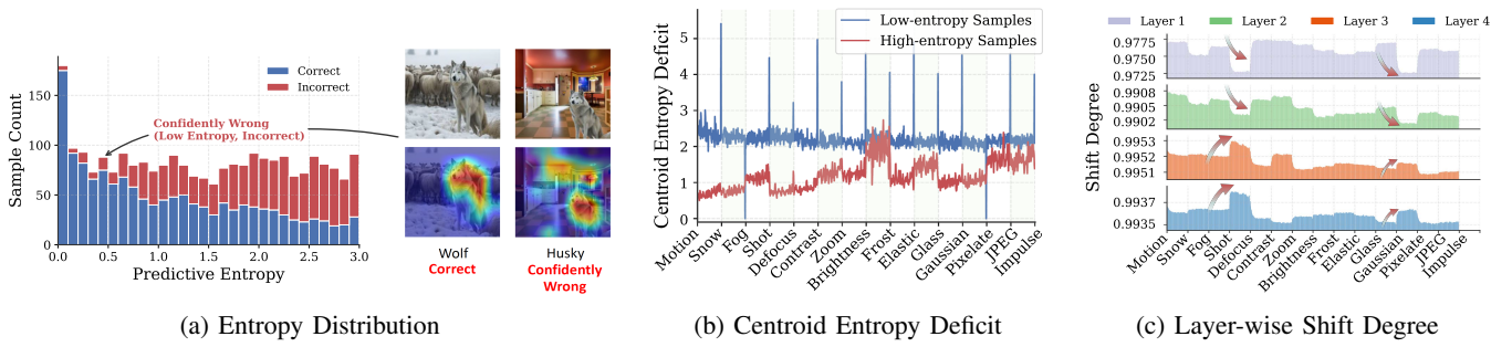
Fig. 2: Why homogeneous TTA fails. (a) Low entropy does not guarantee reliability: even highly confident predictions can be wrong and may be driven by spurious cues. (b) High-entropy samples are weak pseudo-label candidates, but their centroid entropy deficit indicates that they still capture shifting target geometry. Discarding them accelerates representation bias and removes useful structural anchors. (c) Layer drift, measured by KL divergence from the source model, is heterogeneous across depth, with different magnitudes and even opposite trends.
