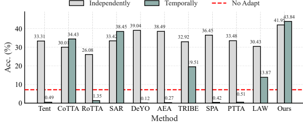
Fig. 10: Static vs. Temporally Correlated Streams. Comparison on ImageNet-C between independently sampled streams (Static setting) and temporally correlated long-horizon streams (Long-horizon T-CS, final round accuracy).
