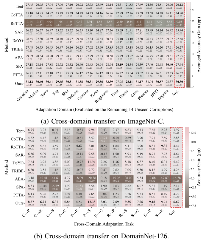
Fig. 11: Cross-domain transfer. (a): ImageNet-C accuracy gains (in percentage points) over No Adapt , averaged across all unseen corruption domains. (b): DomainNet-126 accuracy gains over No Adapt for each cross-domain transfer pair (Adaptation \rightarrow Evaluation, where C: Clipart, P: Painting, R: Real, and S: Sketch). Results are reported as mean \pm standard deviation over five runs.
