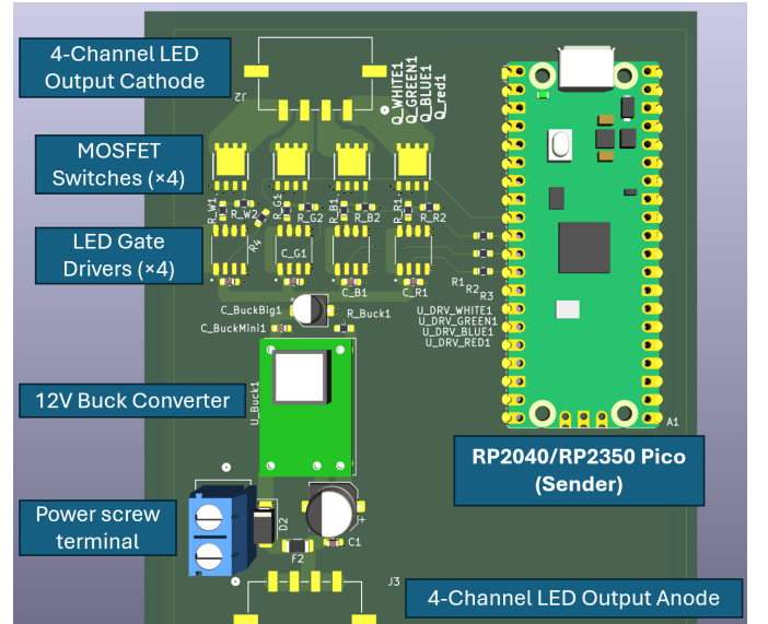
Fig. 2: (b) Sender LED driver PCB: RP2040/RP2350 Pico, TC4420COA gate drivers ( \times 4 ), SIR800DP-T1-GE3 MOSFETs ( \times 4 ), PTN78000WAH 12 V \rightarrow 5 V module, and 4-channel LED terminal blocks.
