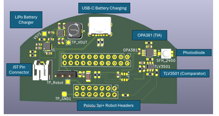
Fig. 1: (a) Receiver analog front-end PCB: OPA381AIDGKT TIA, SFH2400-Z photodiode, TLV3501AIDBVR comparator, MCP4725 DAC, TPS63031 3.3 V regulator, BQ24074 LiPo charger, Pololu 3pi+ robot headers, and USB-C charging port.
