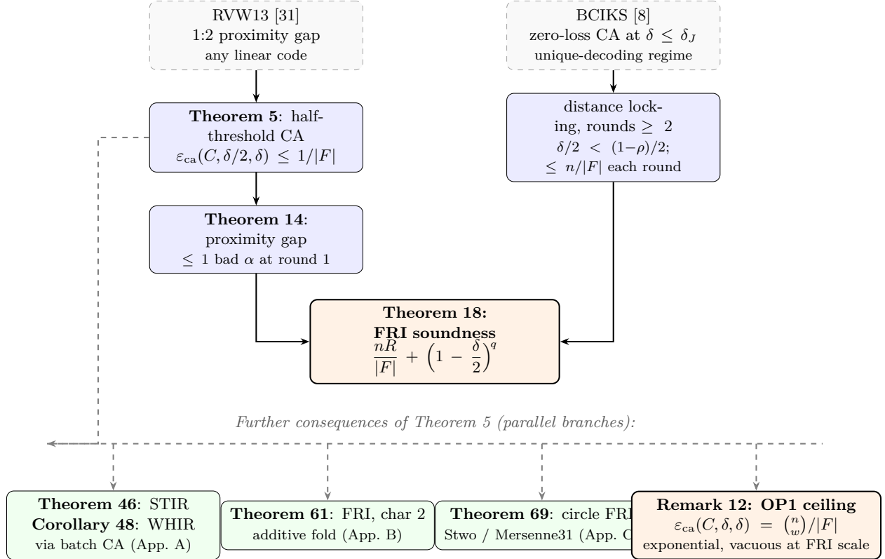
Figure 1: Proof map. Top half (mainline): RVW13 yields the half-threshold CA bound (Theorem 5), which composes with the FRI even/odd coupling to give the round-1 proximity gap (Theorem 14); BCIKS supplies the round- \geq 2 distance lock (the structural observation \delta/2 < (1-\rho)/2 ); the two combine into the FRI soundness theorem. Bottom half (parallel branches from the same CA bound): STIR/WHIR via batch CA; characteristic-2 FRI via additive coupling; circle FRI via the Stwo coupling; equal-threshold CA (the OP1 ceiling) showing the \binom{n}{w}/|F| bound is vacuous at FRI scale, so the 2\times overhead is intrinsic to any CA-based proof. The list-size structural track (§7) is independent of the soundness proof and is not shown.
